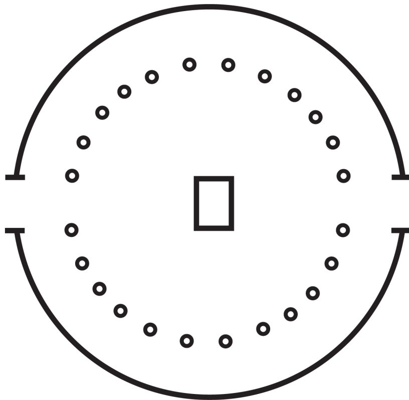
Celtic Round House Floor Plan
