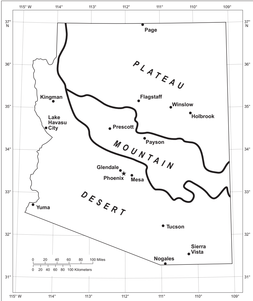
Landform Regions of Arizona
