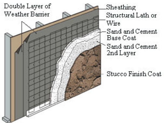
Layers in a Stucco Home
